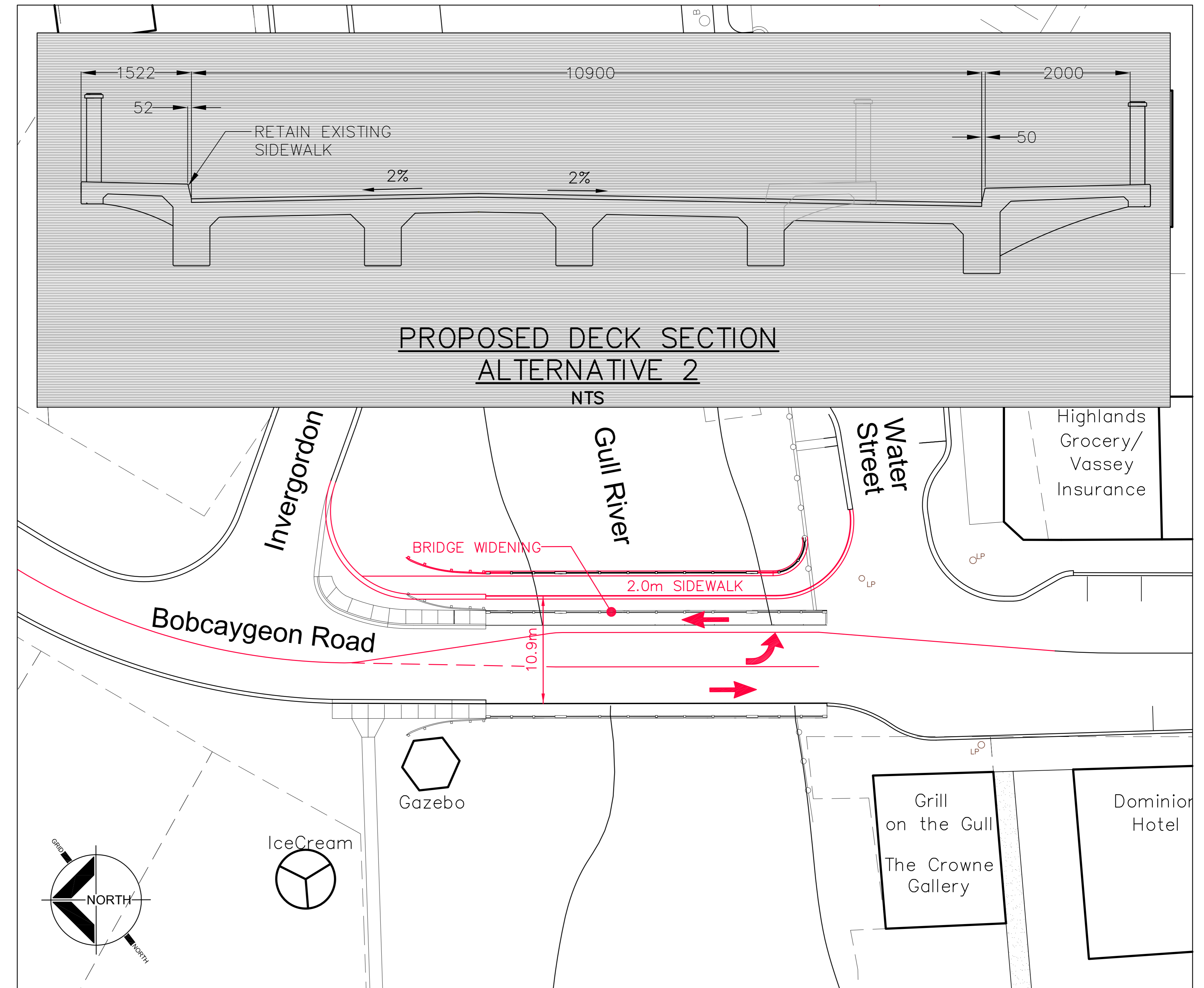
Bridge Alternative 2 (widen bridge to three lanes and widen east sidewalk) - 1:500
