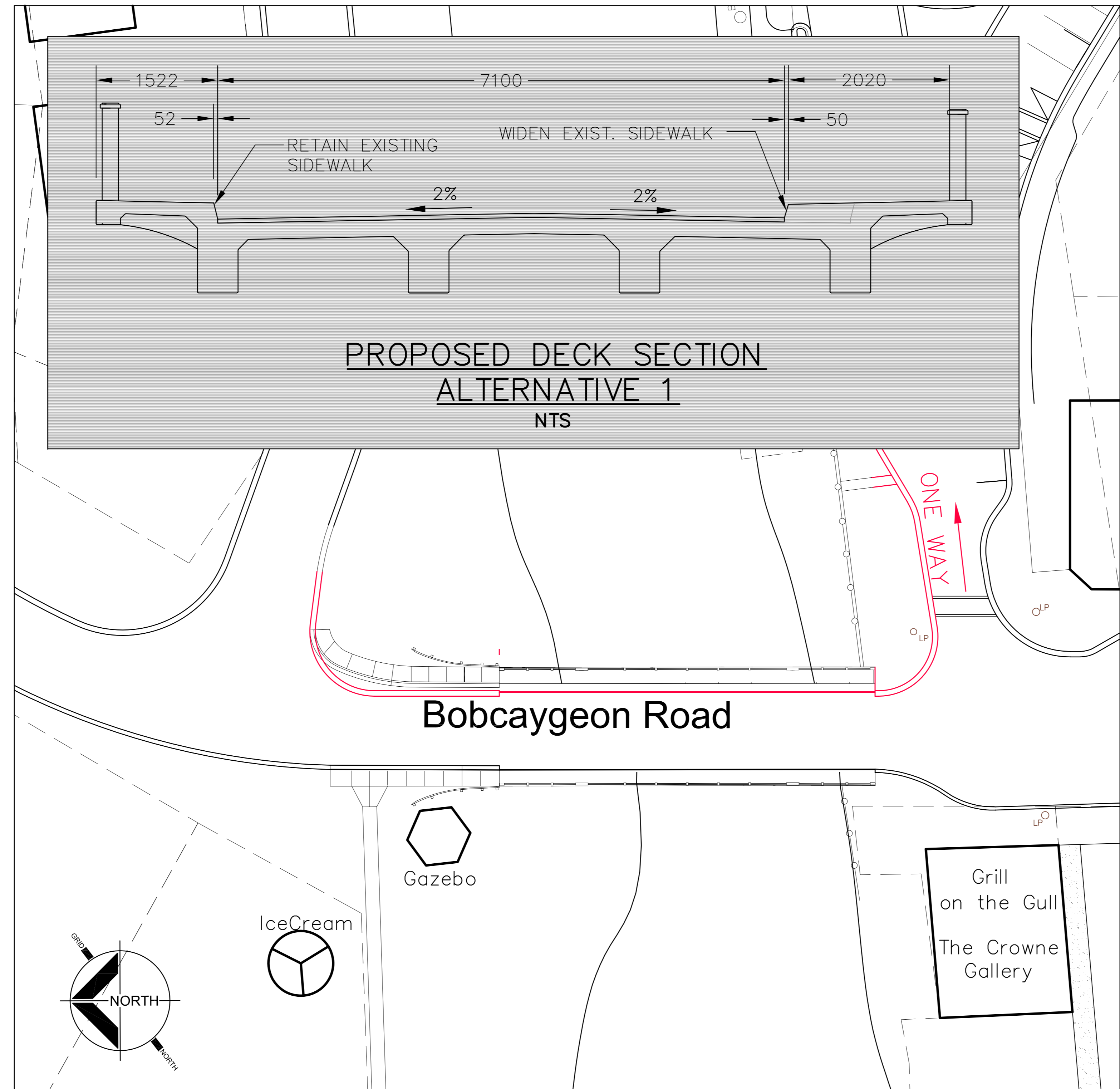
Bridge Alternative 1 (low cost - widen east sidewalk reduce lane width) - 1:500
