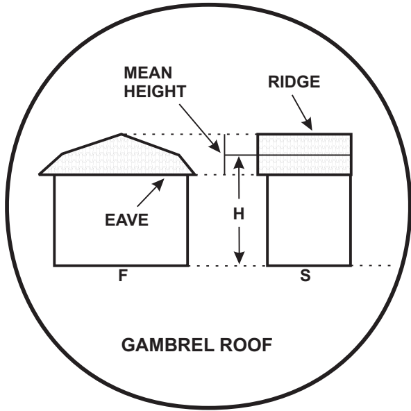
FIGURE 3 - ILLUSTRATIONS OF BUILDING HEIGHT
